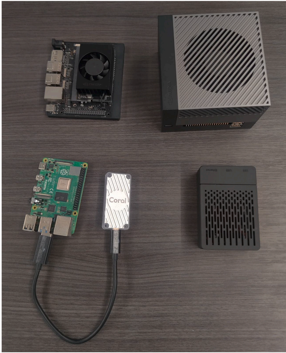
Fig. 3. The analyzed Edge devices used for the Edge-AI system. Top left: NVIDIA Jetson Orin Nano, Top right: NVIDIA Jetson AGX Orin, Bottom left: RPI 4 Model B with Google Coral, Bottom right: RPI 4 Model B.
