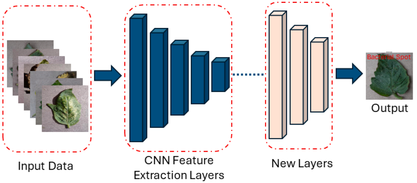
Fig. 2. Overall process of employing different CNN-based deep learning networks (extracting CNN features and addition of new layers) for tomato leaf diseases detection.
