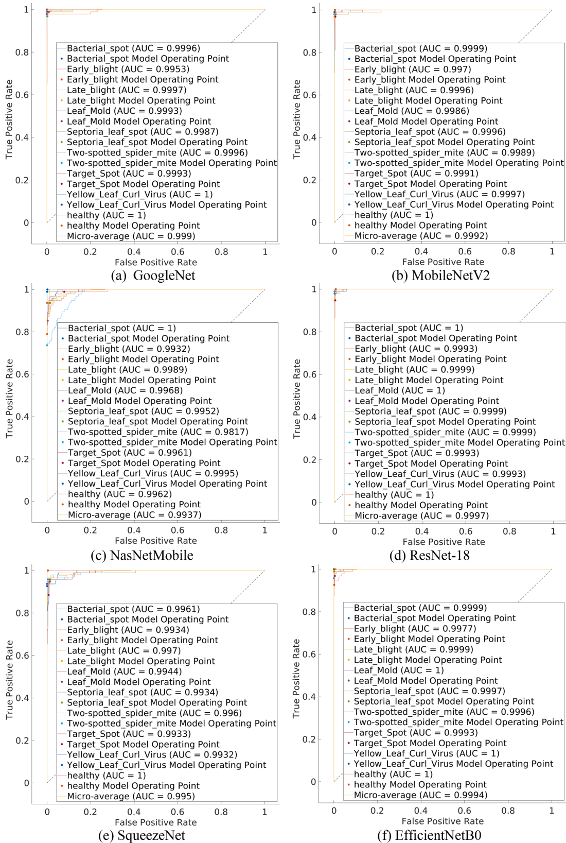
Fig. 6. ROC (receiver operator characteristic) curves representing the sensitivity (true positive rate) against the specificity (false positive rate) of GoogleNet (a), MobileNetV2 (b), NasNetMobile (c), ResNet-18 (d), SqueezeNet (e), and EfficientNetB0 (f).
