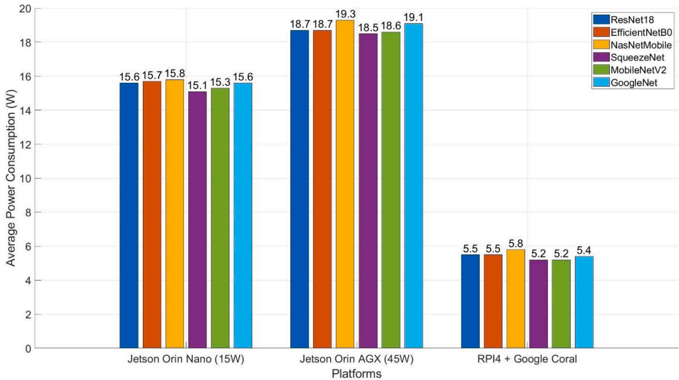
Fig. 9. Average Edge device power consumption observed across various CNN models during algorithm execution.
