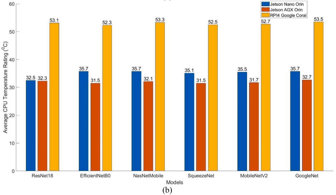
Fig. 8. Resource utilization (both GPU and CPU) (a) and average CPU temperature rating (b) for all CNN networks running on Edge devices (NVIDIA Jetson Nano Orin, NVIDIA AGX Orin, and RPI 4 with and without Google Coral).
