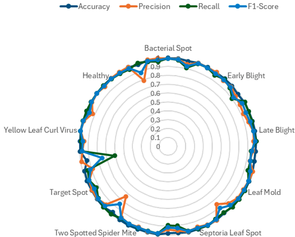
Fig. 5. Accuracy, precision, recall and F1-score of each tomato leaf disease category. CNN networks can be read as clockwise in the order of GoogleNet, MobileNetV2, SqueezeNet, NasNetMobile, EfficientNetB0, and ResNet-18.
